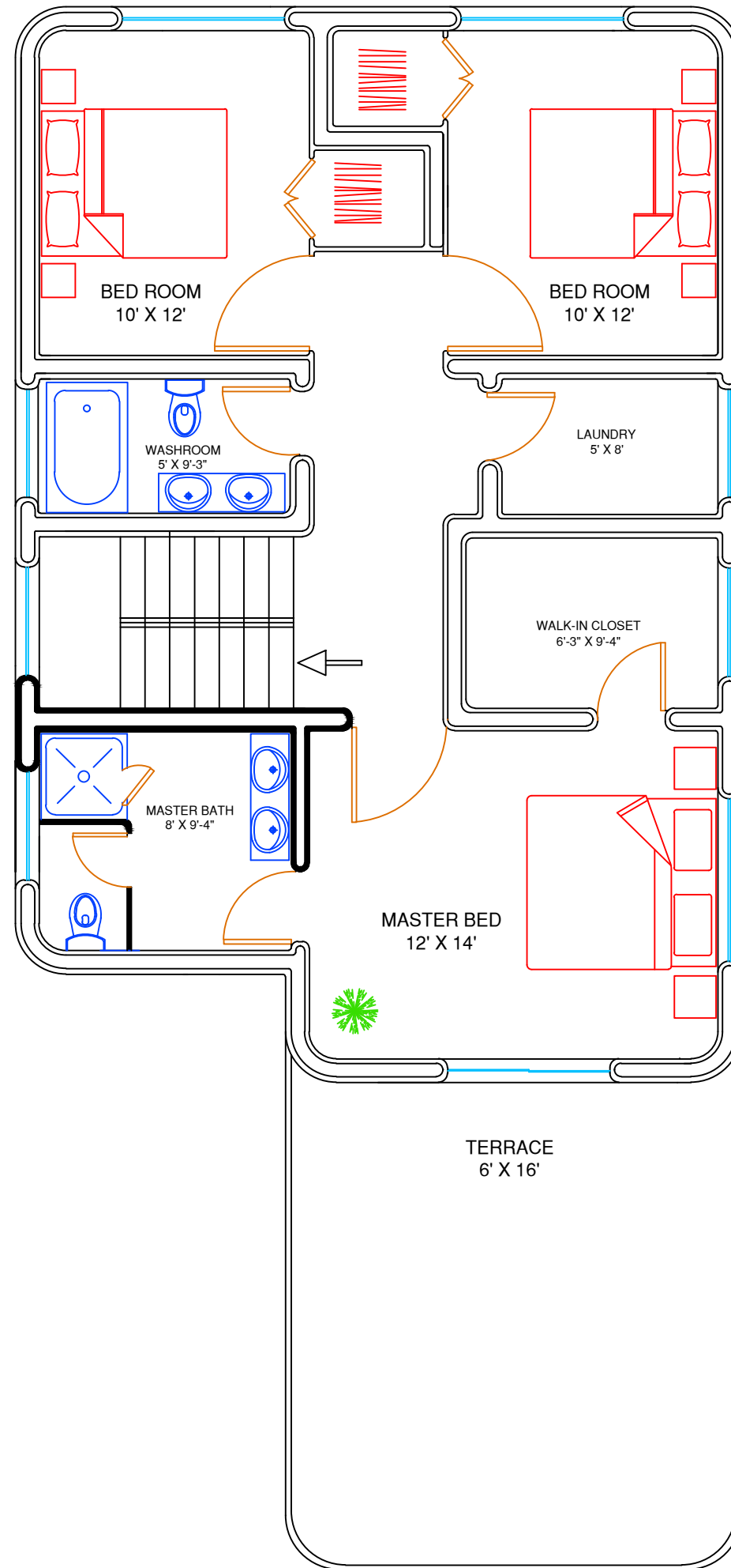
FIRST FLOOR
