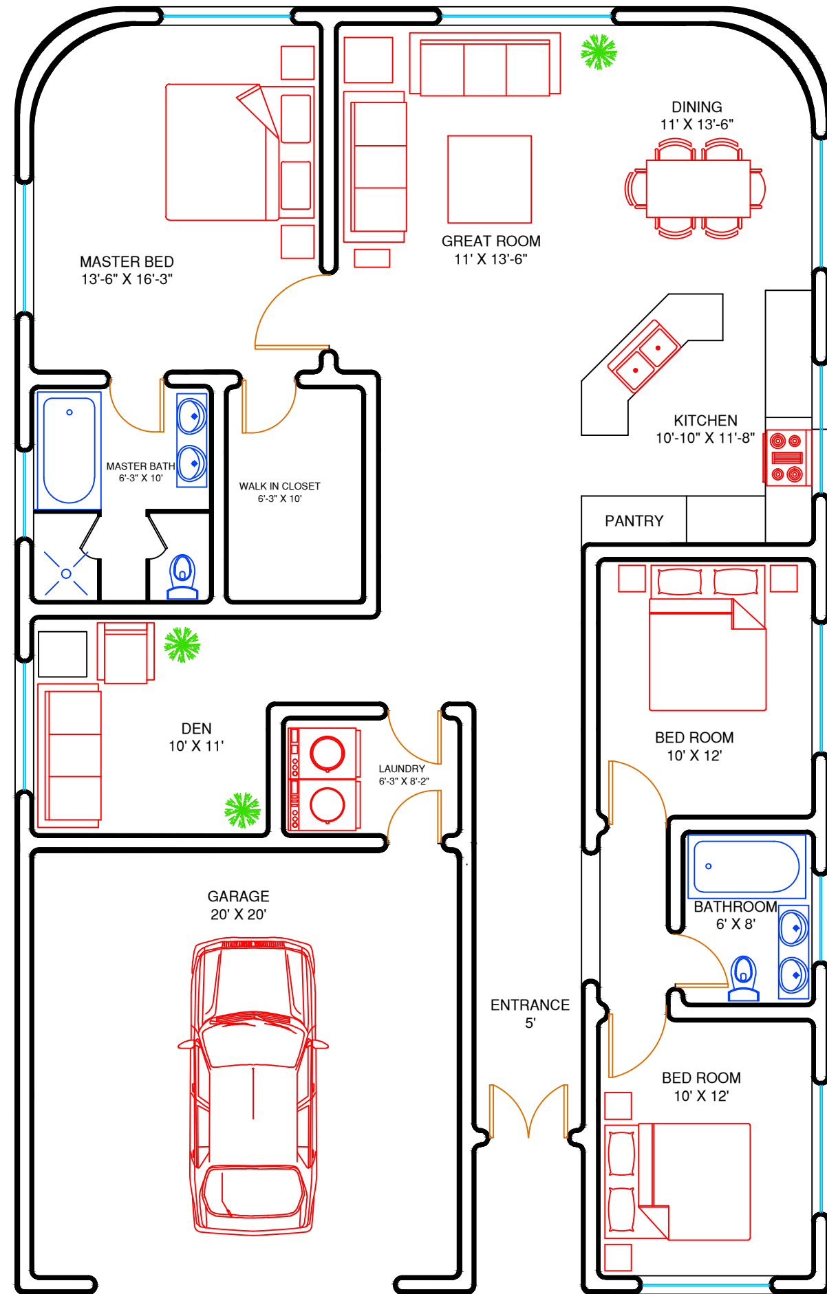
FLOOR PLAN- SINGLE STOREY
